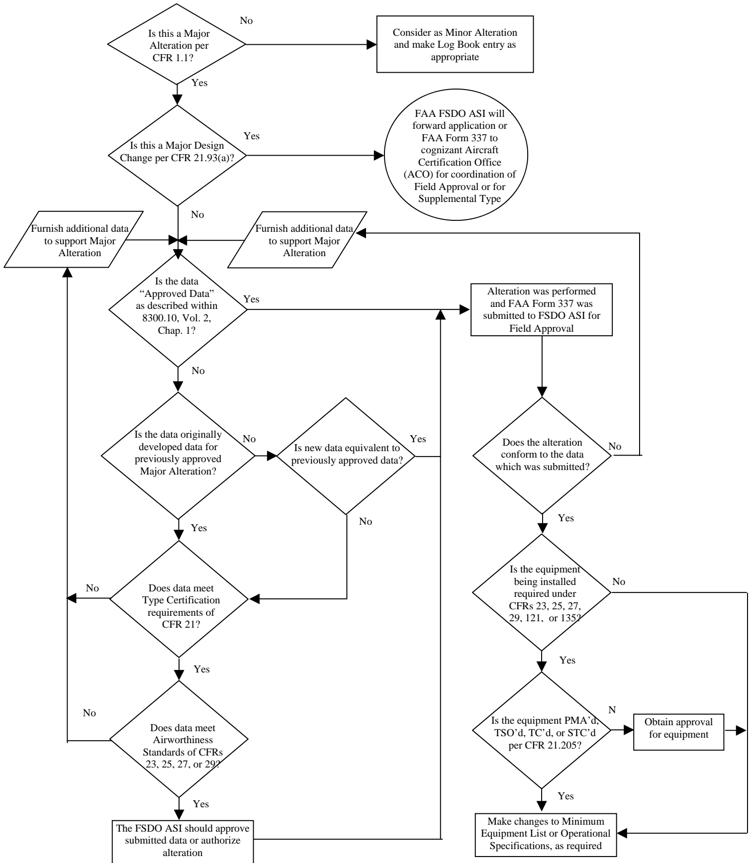
FIGURE 1-2. DECISION FLOW CHART FOR FIELD APPROVAL PROCESS
