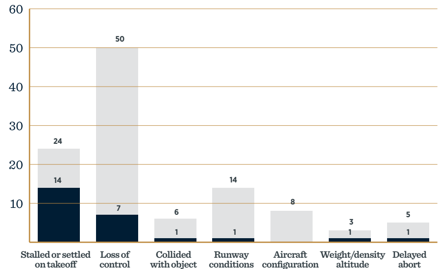
FIGURE 22. TYPES OF TAKEOFF AND CLIMB ACCIDENTS
