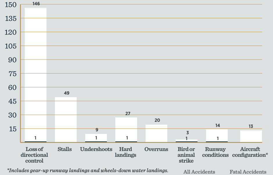
FIGURE 36. TYPES OF LANDING ACCIDENTS
